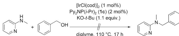
Scheme 4. N -Alkylation of secondary amines with benzyl alcohol.
