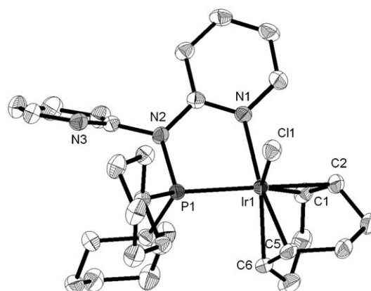
Figure 1. Molecular structure of monomeric [(\text{Py}_2\text{NPCy}_2)\text{Ir}(\text{cod})\text{Cl}] ( 2 ). Selected bond lengths [Å] and angles [°]: N1–Ir1 2.118(3), P1–Ir1 2.3024(11), Cl1–Ir1 2.5707(10), C1–Ir1 2.112(4), C2–Ir1 2.157(4), C5–Ir1 2.137(4), C6–Ir1 2.153(4), C1–C2 1.427(6), C5–C6 1.406(7), N1–Ir1–P1 80.57(10), P1–Ir1–Cl1 96.52(4), N1–Ir1–Cl1 85.31(9), C1–Ir1–C2 39.04(17), C5–Ir1–C6 38.26(17), C1–Ir1–N1 88.03(16), C2–Ir1–Cl1 98.48(13), C6–Ir1–P1 89.45(12), C5–Ir1–Cl1 82.71(13).
