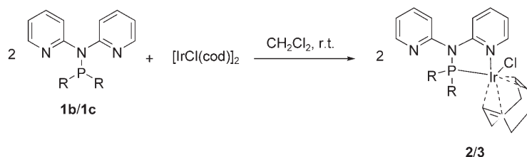
Scheme 2. Synthesis of 2 (R = cyclohexyl) and 3 (R = isopropyl).
