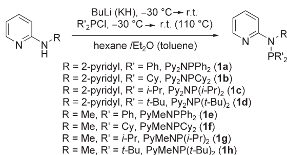
Scheme 1. Synthesis of the used P,N ligands.
